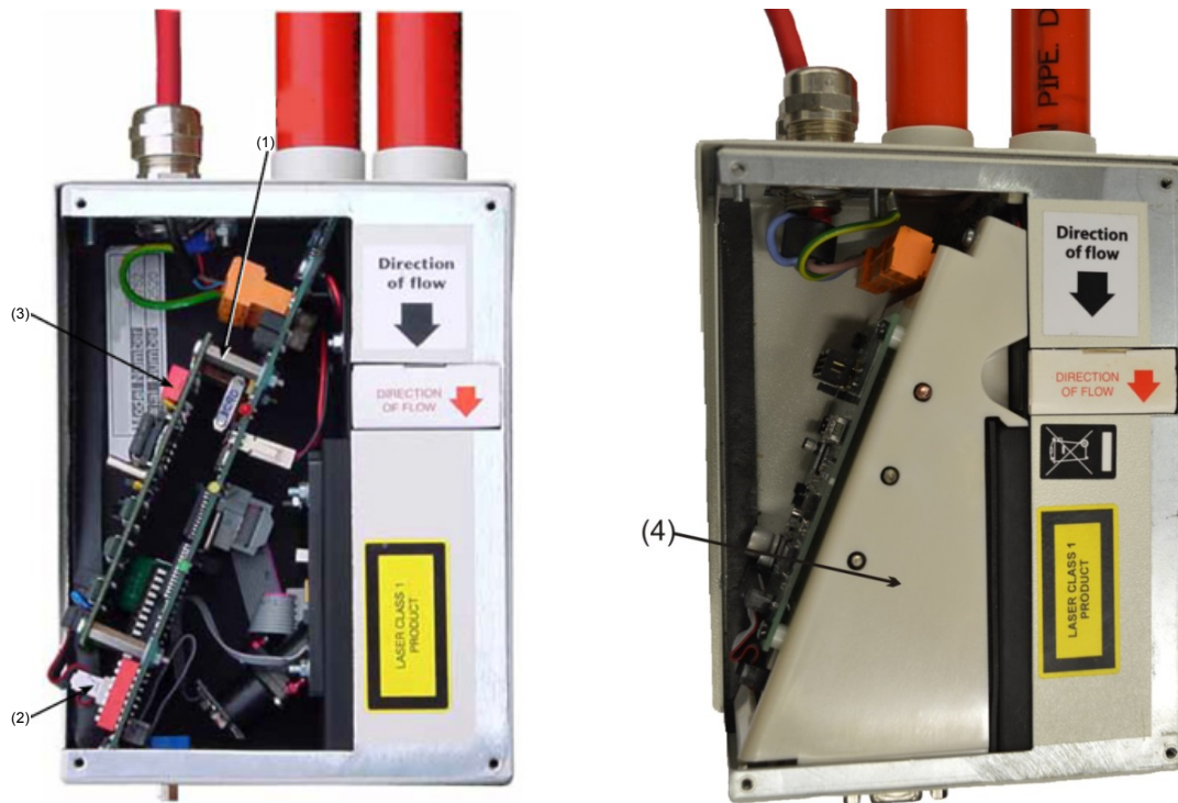
Figure 13: APIC connections (EN/UL certified models)
