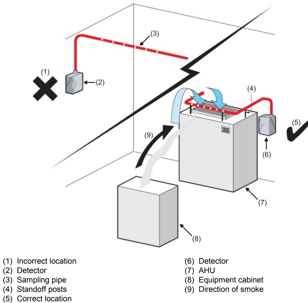
Figure 5: Air handling unit in vicinity of the detector (exhaust shown for clarity)
